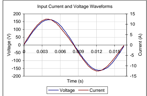
Input AC Current Waveform (ITHD = 3.65%, 50% Load)
