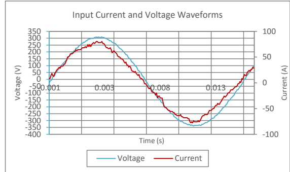
Input AC Current Waveform (ITHD = 5.37%, 50% Load)
